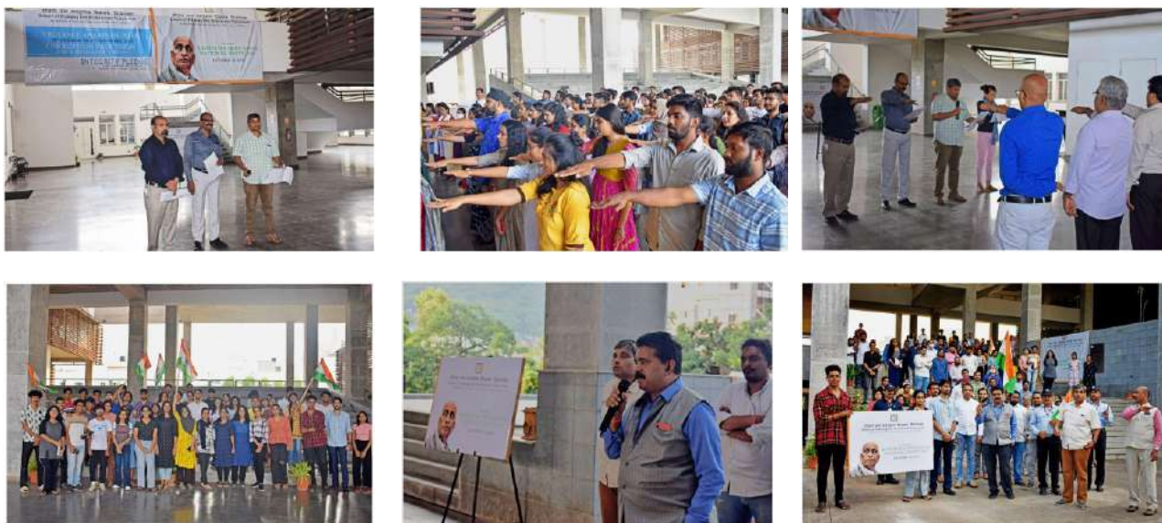
Figure 20. Integrity Pledge
